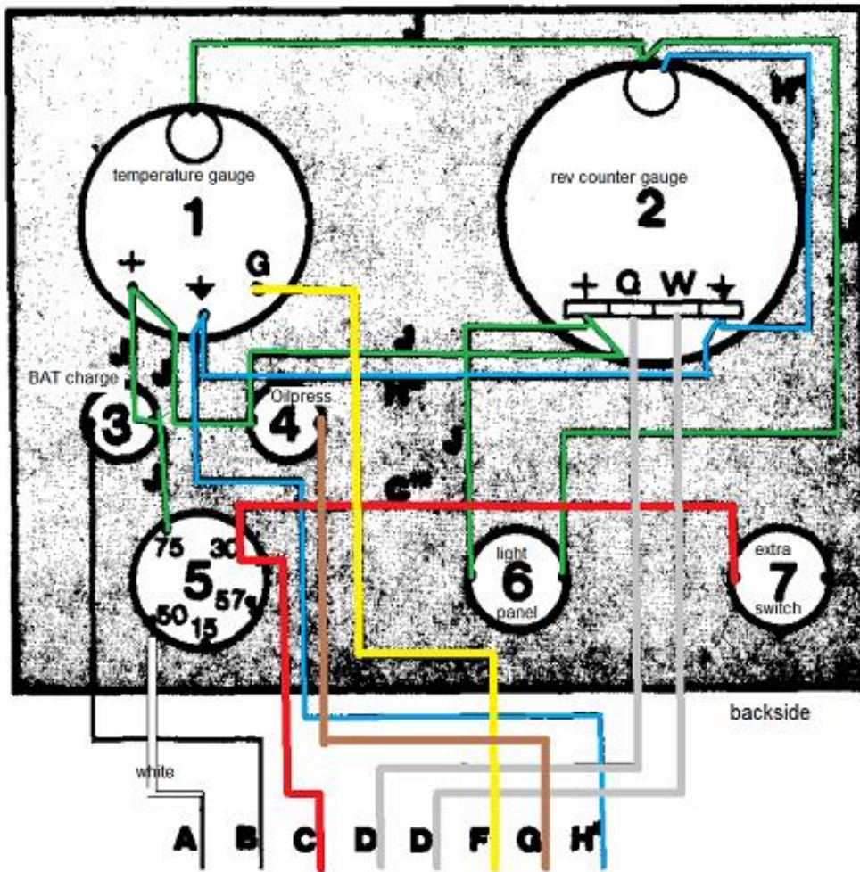
Volvo penta motor console wiring diagram (colour)
